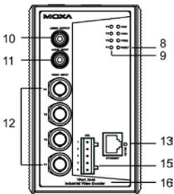
VPort 364A-M-SC Front Panel View
