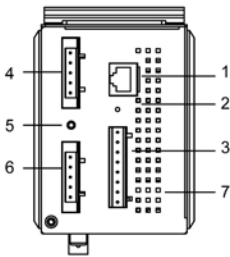
VPort 364A Front Panel View
